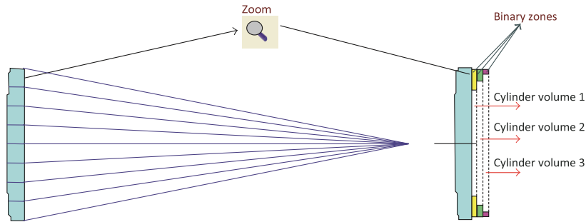
Fig. 4: The binary diffractive lens with discrete phase levels.
