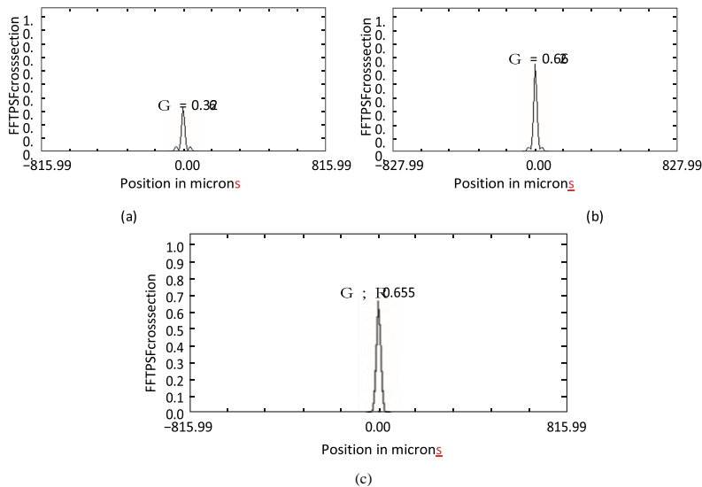
Fig. 5: FFT PSF cross sections of (a) refractive lens, (b) diffractive lens, and (c) designed binary lenses.
